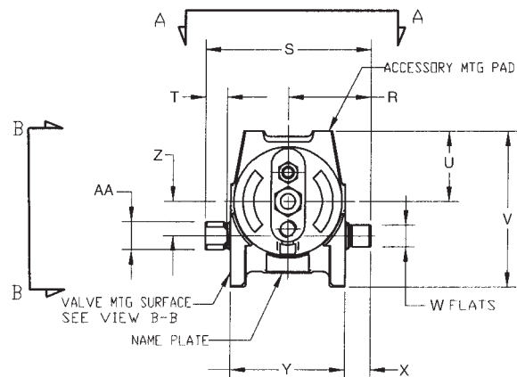
END VIEW REPRESENTATIVE OF ALL MODELS
